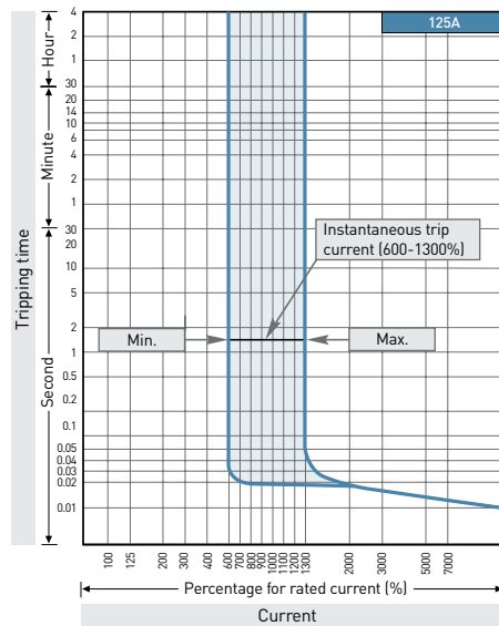
Tripping curves
