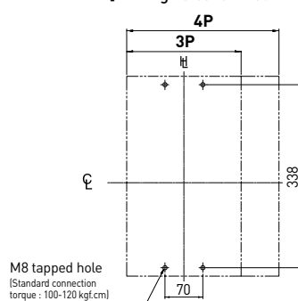
[Drilling holes for mounting]
