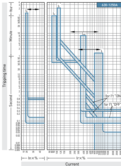
Tripping curves
