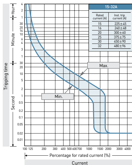
Tripping & temperature derating curves
