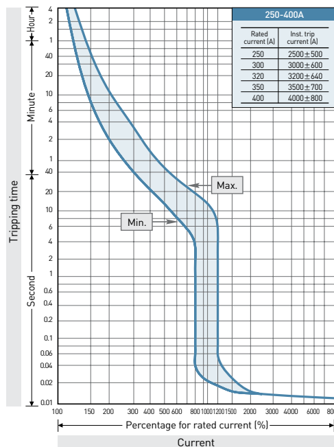
Tripping & temperature derating curves
