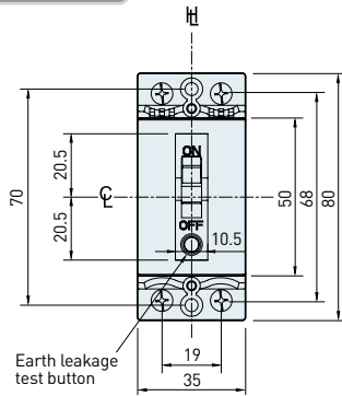
UMG30Sg / UMG50Sg
