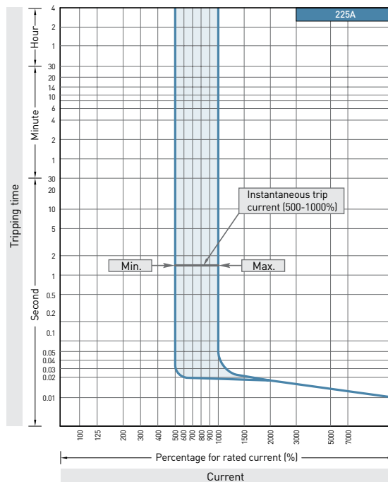
Tripping curves
