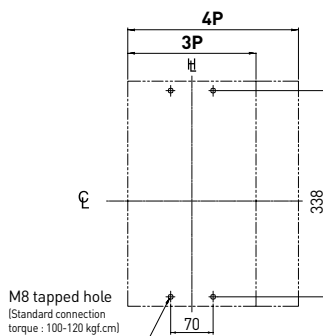
[Drilling holes for mounting]
