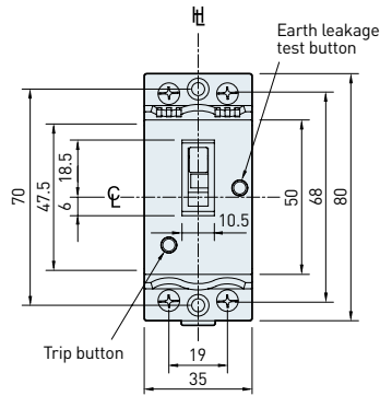
UMG30Hg / UMG50Hg
