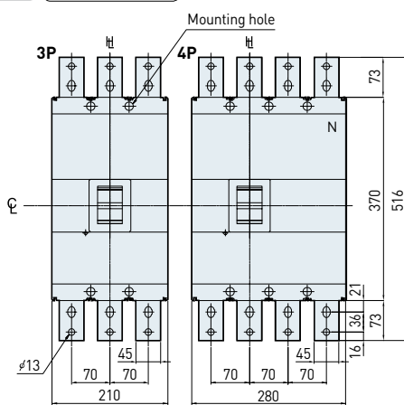
[Drilling holes for mounting]
