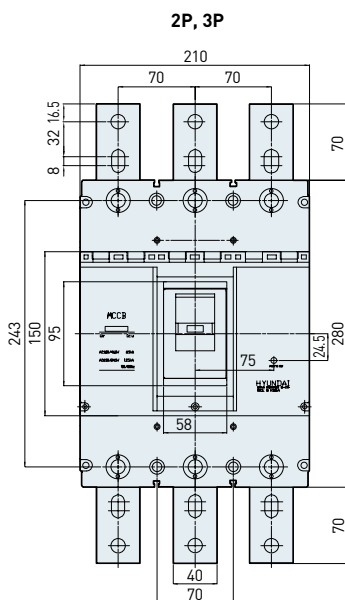
[Terminal part]
