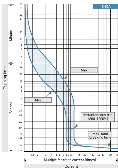
Tripping & temperature derating curves
