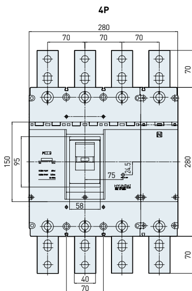
[Connection conductor]
