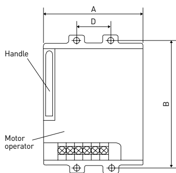
[MOT-10/20/40/68/80/12/46]
