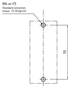
UMG30Hg / UMG50Hg
